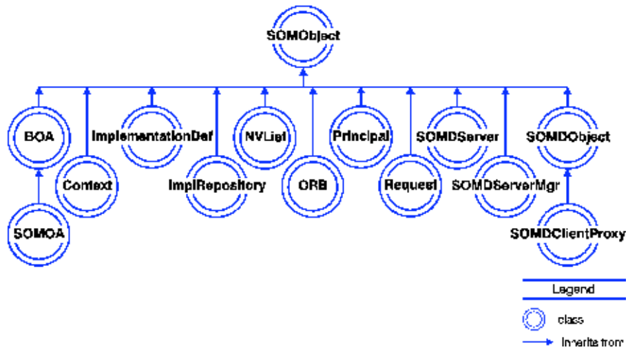
Figure 2. DSOM Framework Organization.
