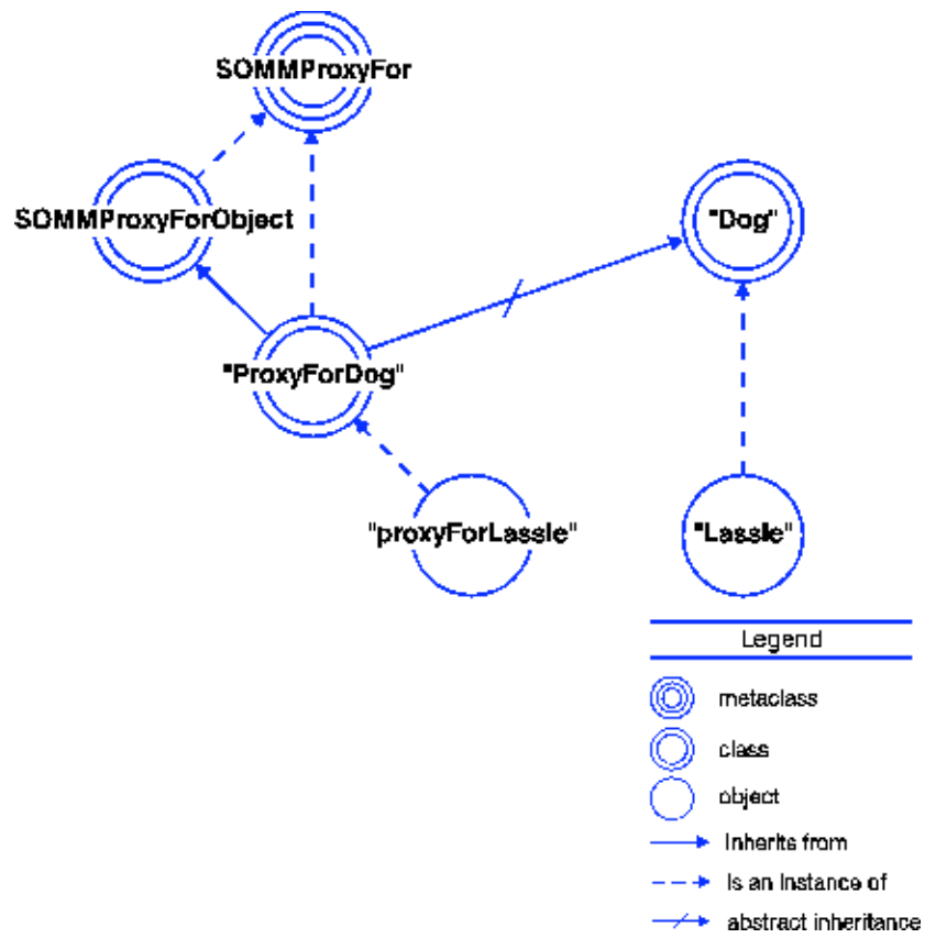
Figure 7. sommMakeProxyClass Method
